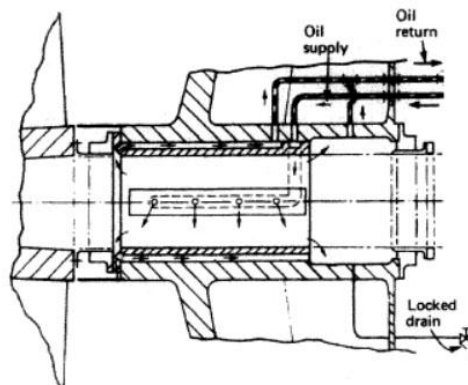
Oil lubricated sterntube bearing
